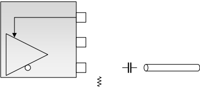
AC-Coupled LVPECL - Thevenin Termination
