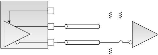
DC-Coupled LVPECL - Thevenin Termination
